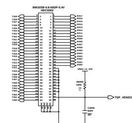
60pin TSP Con.
