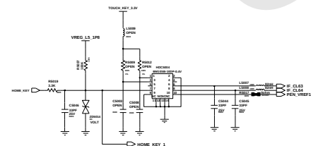
Home KEY & KEY LED Conn
