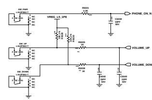
POWER & VOLUME KEY
