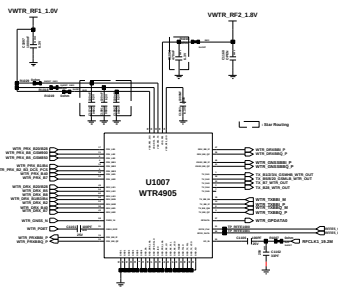
TRANSCEIVER
