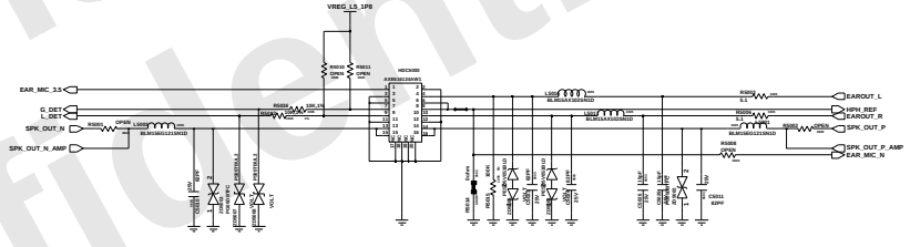
Earjack
