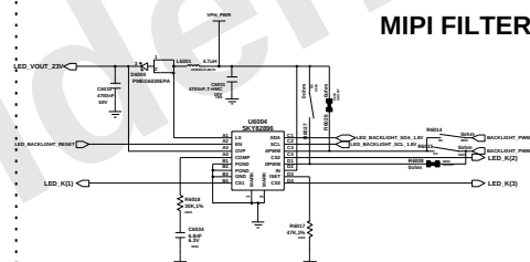
LED BACKLIGHT DRIVER IC
