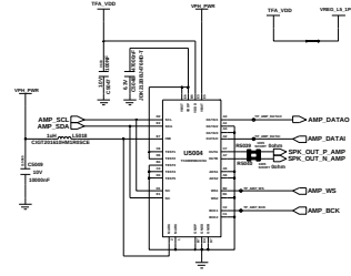
Audio AMP
