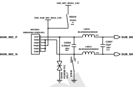
SUB MIC
