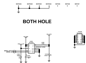
APT MODULATOR
