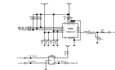
GRIP SENSOR
