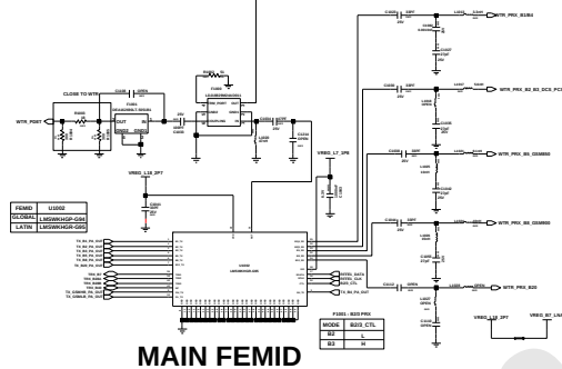
MAIN FEMID
